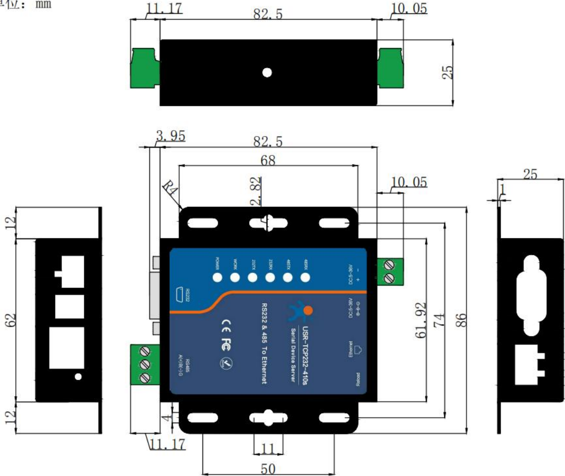
410S外观尺寸图
